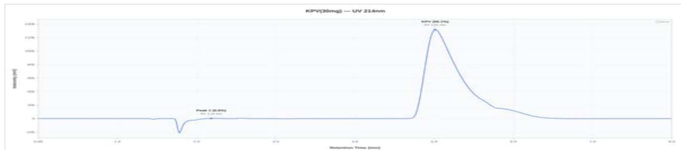
KPV 30mg - KPV: UV Chromatogram
